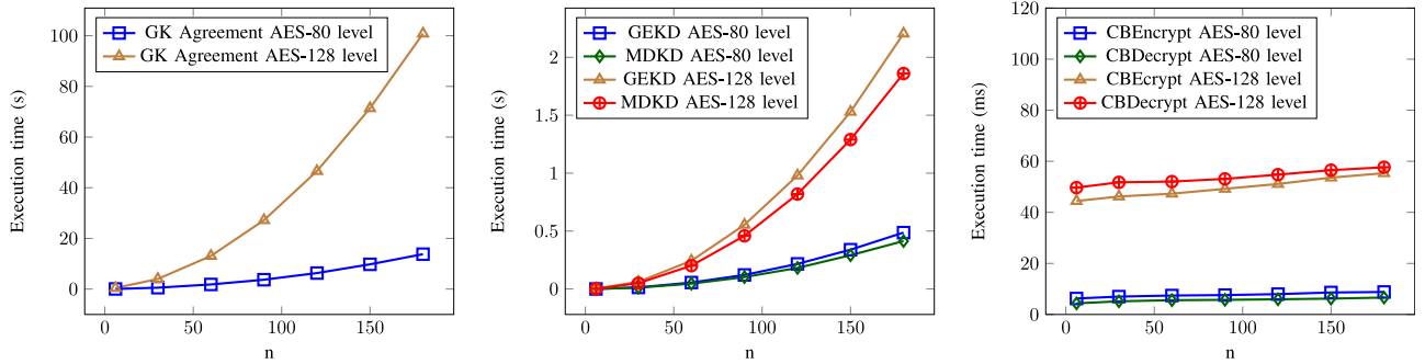
Fig. 1. Execution time of group key agreement, group encryption key derivation, member decryption key derivation, CBEncrypt, and CBDDecrypt for AES-80 and AES-128 levels.
