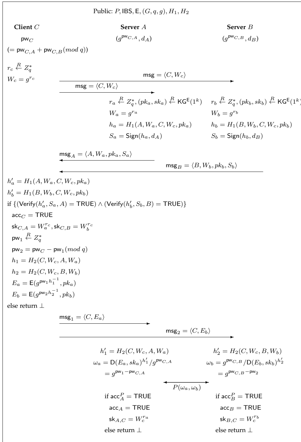
Fig. 1. ID2S PAKE protocol P' based on IBS
