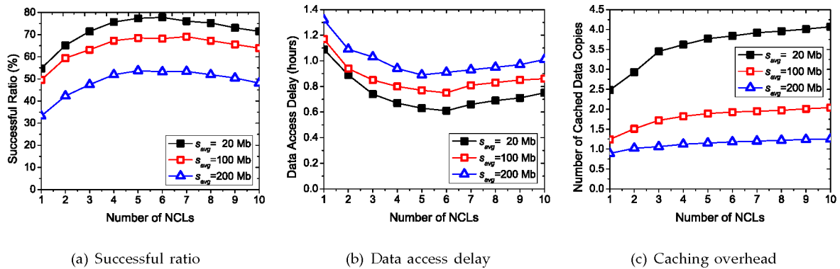
Fig. 16. Performance of data access with different number of NCLs.
