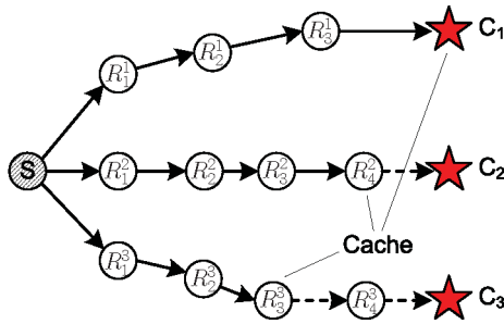
Fig. 7. Determining caching location at NCLs.
