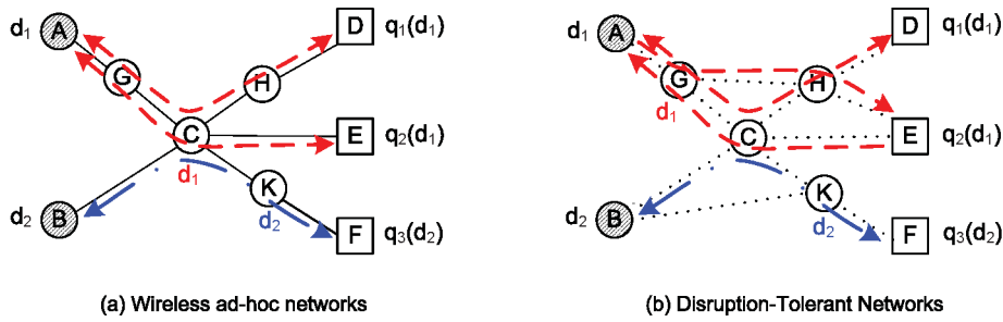
Fig. 1. Caching strategies in different network environments. Data d_1 generated by node A are requested by nodes D and E , and d_2 generated by node B are requested by node F . A solid line in (a) between nodes indicates a wireless link, and a dotted line in (b) indicates that two nodes opportunistically contact each other.
