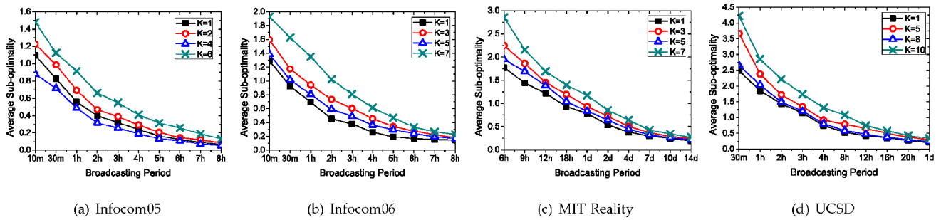
Fig. 6. Suboptimality of distributed NCL selection on realistic DTN traces.
