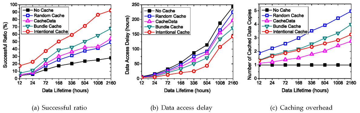
Fig. 13. Performance of data access with different data lifetime.
