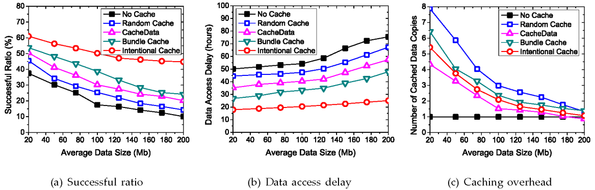
Fig. 14. Performance of data access with different node buffer conditions.
