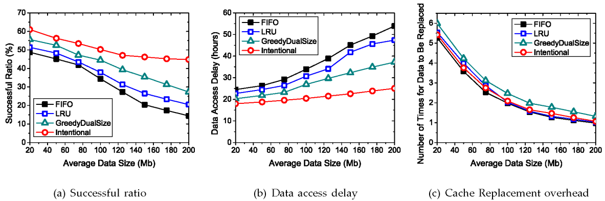
Fig. 15. Performance of data access with different cache replacement strategies.
