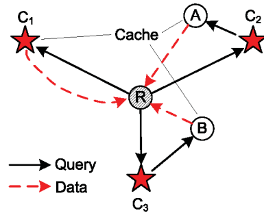
Fig. 8. Pulling data from the NCLs.
