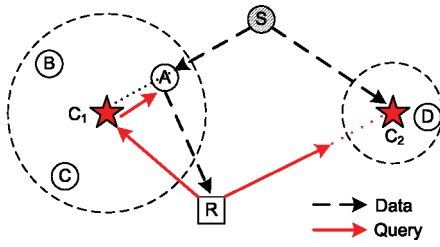
Fig. 2. The big picture of intentional caching.
