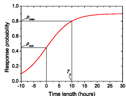
Fig. 9. Probability for deciding data response.
