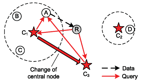
Fig. 11. NCL load balancing.
