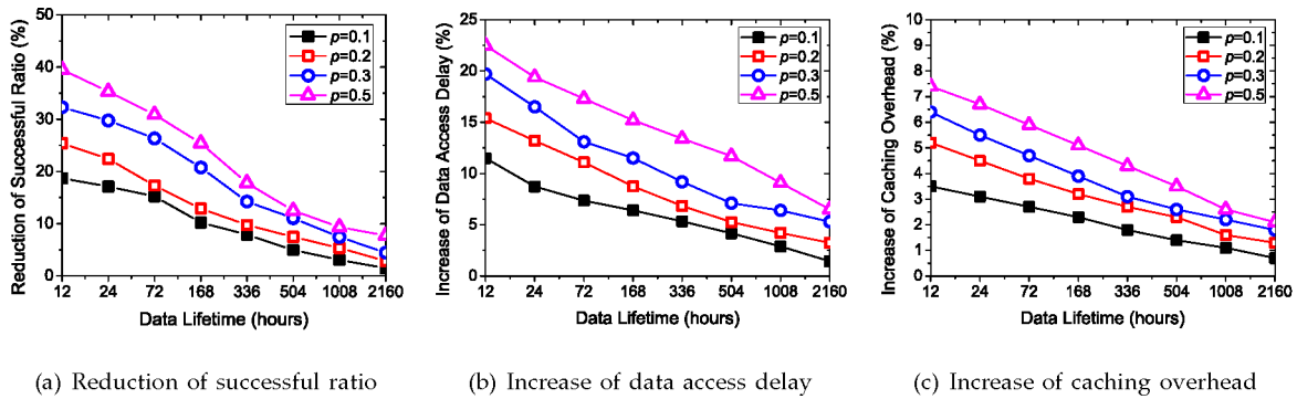
Fig. 17. Impact of NCL load balancing on the caching performance.
