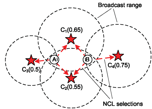
Fig. 5. Inconsistency in distributed NCL selection when K = 3 .
