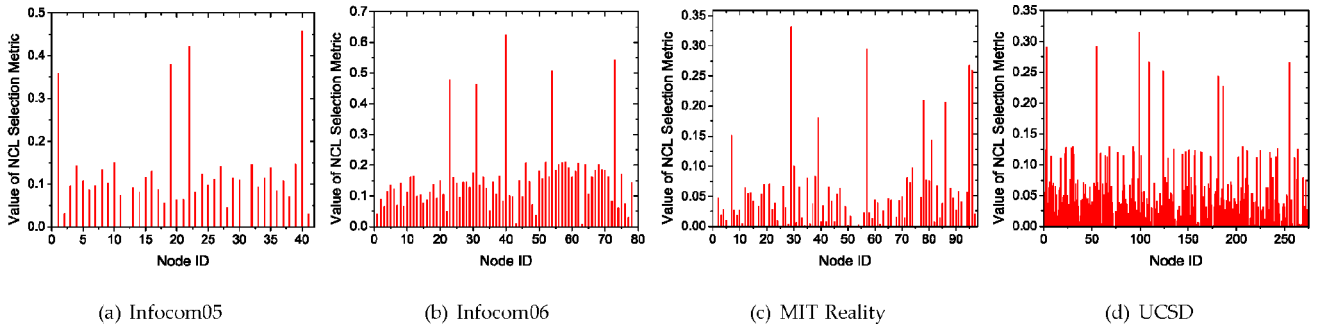
Fig. 4. Values of NCL selection metric on realistic DTN traces.
