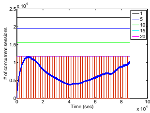
Fig. 5. Maximum cost: Total # sessions needed with a 15 sec ICC pulse width - Synthetic trace, deadline for VoD in secs shown in legend
